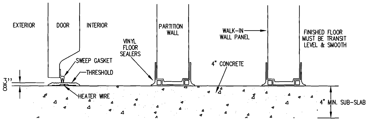
VINYL FLOOR SEALERS ON TOP OF UNINSULATED FLOOR
