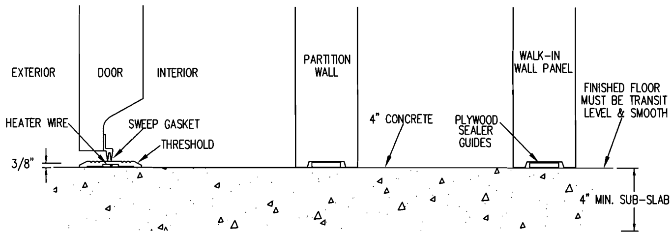
FEMALE BOTTOM RAILS ON TOP OF UNINSULATED FLOOR DETAIL 003B BD 7/9/01
