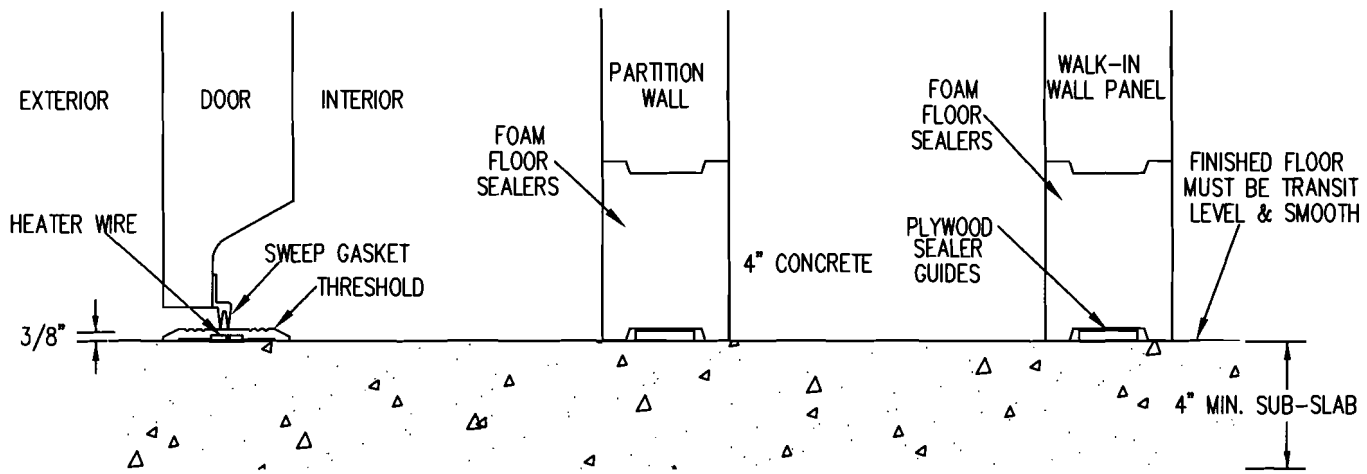
FOAM FLOOR SEALERS ON TOP OF UNINSULATED FLOOR
