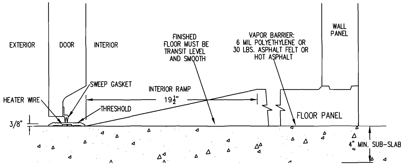
INTERIOR RAMP FLOOR DETAIL
