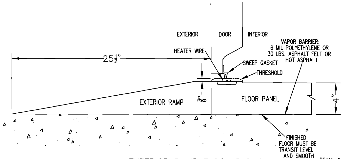
EXTERIOR RAMP FLOOR DETAIL
