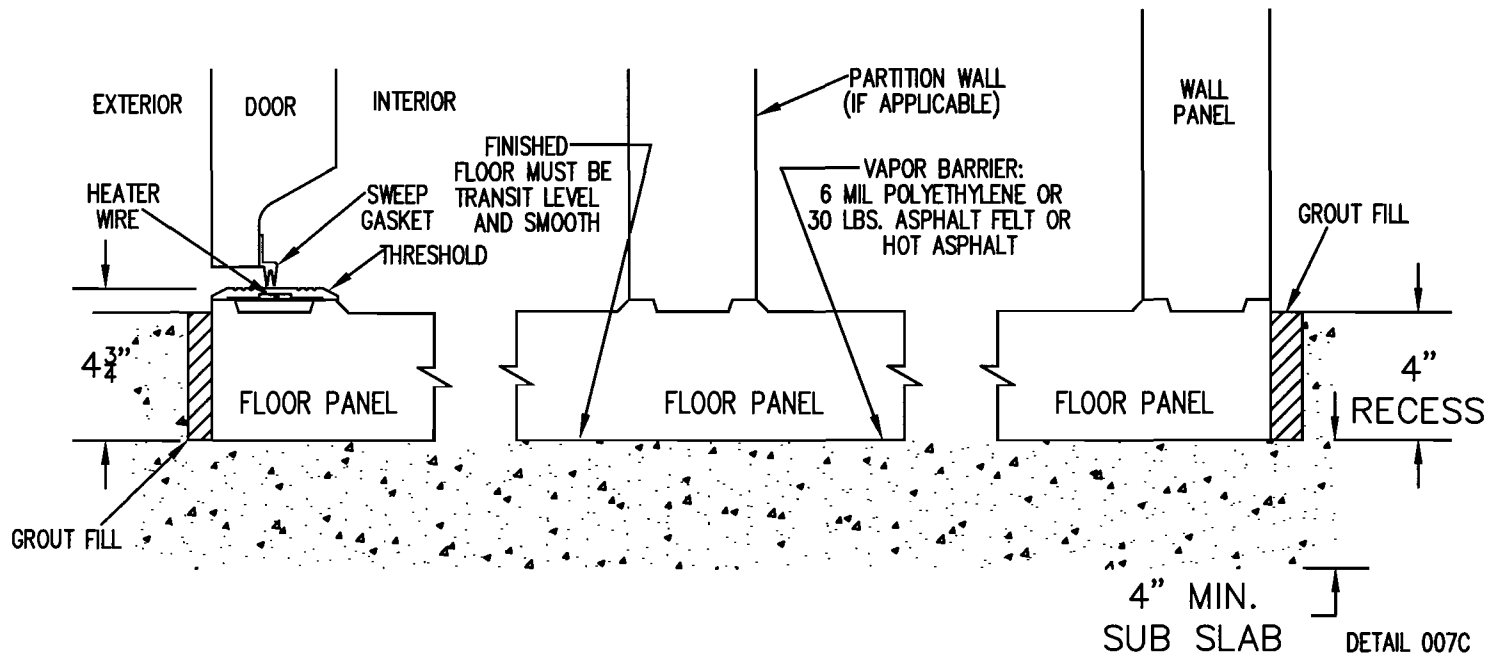
STD. WITH FLOOR DETAIL IN A 4" RECESS
