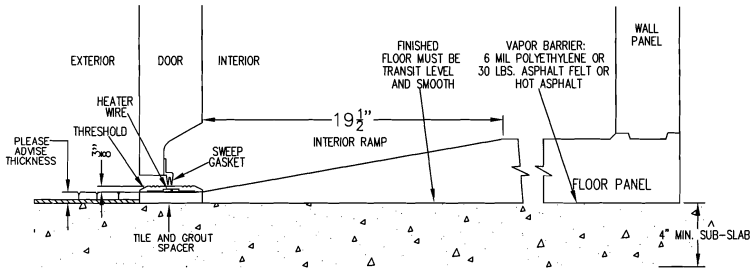
INTERIOR RAMP FLOOR DETAIL HELD UP FOR TILE AND GROUT FINISHED FLOOR ON EXTERIOR OF WALK-IN
