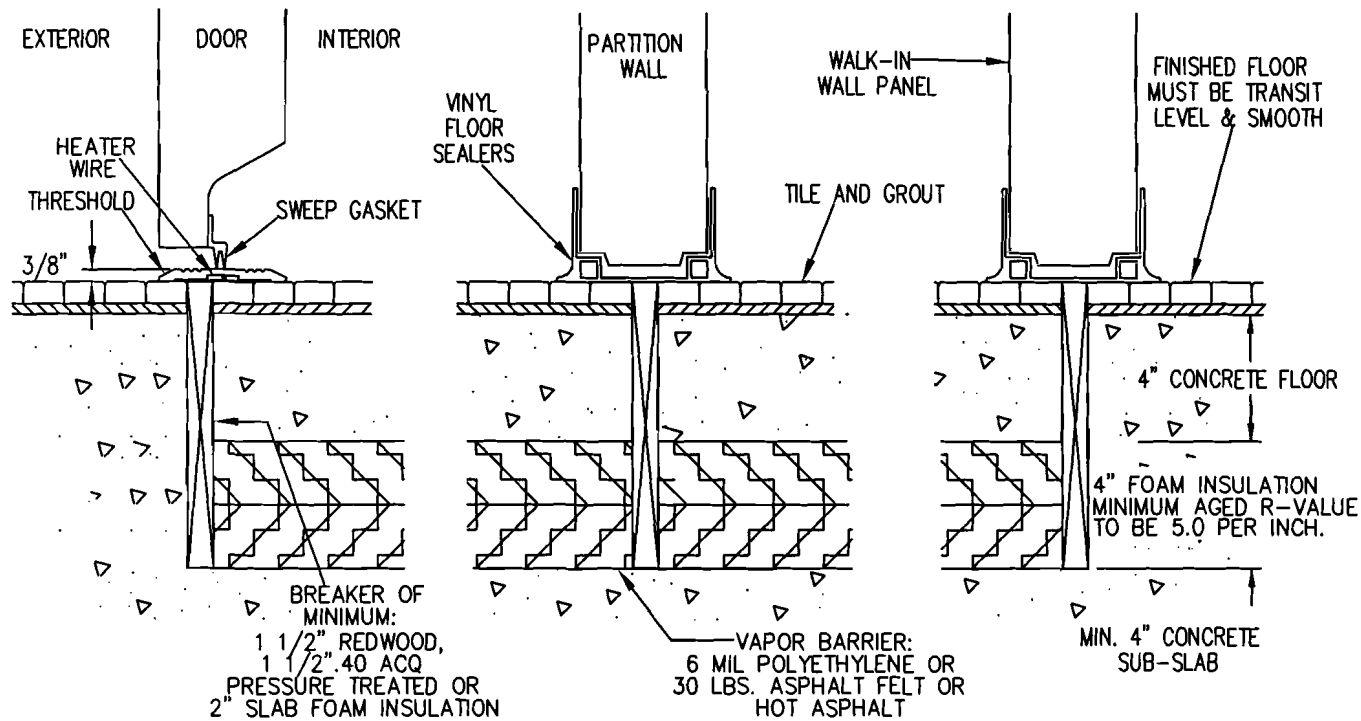
VINYL FLOOR SEALERS ON TOP OF AN INSULATED FLOOR WITH TILE AND GROUT (BEFORE WALK-IN INSTALLATION)
