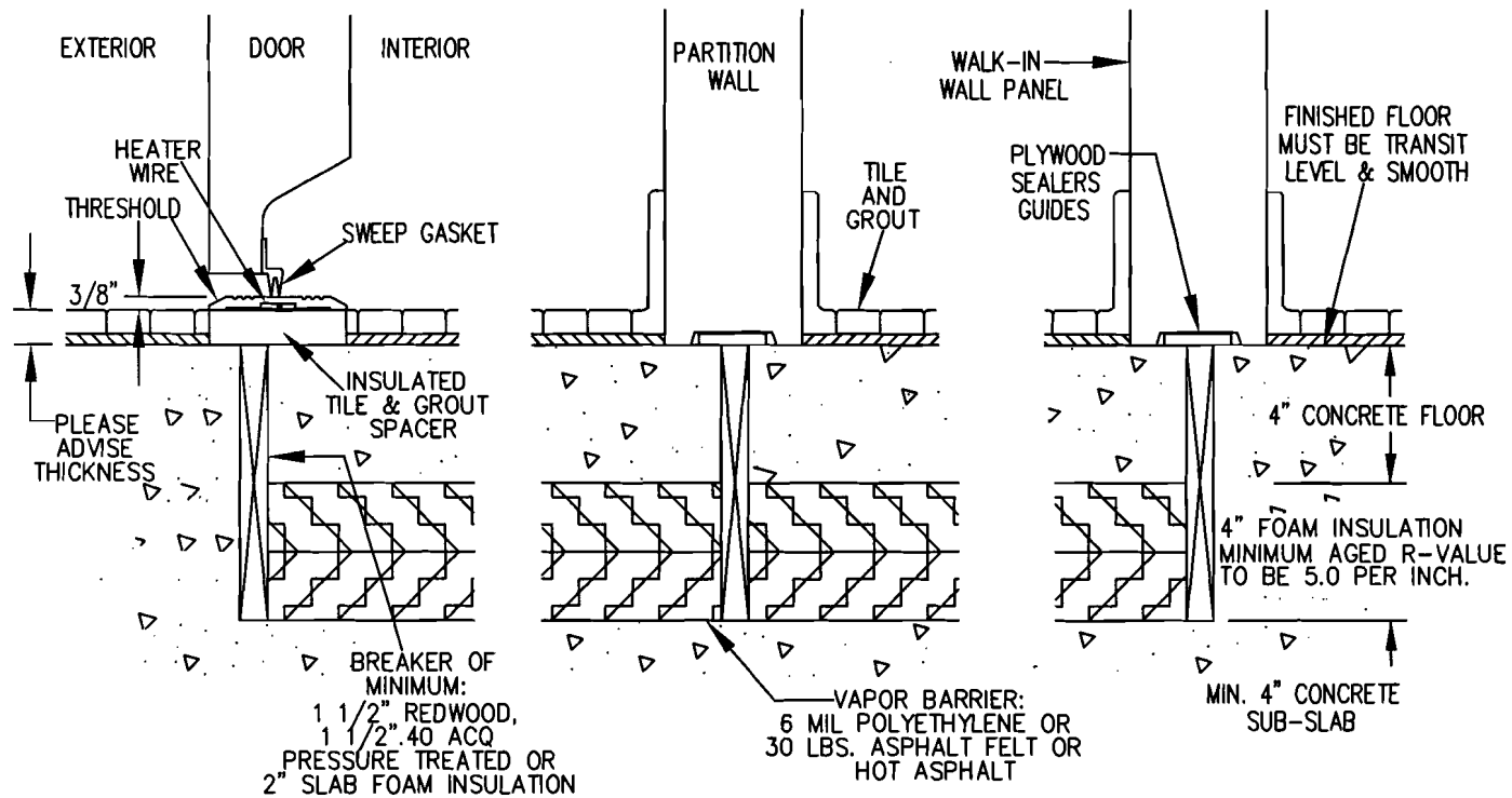
FEMALE BOTTOM RAILS ON TOP OF AN INSULATED FLOOR WITH TILE AND GROUT (AFTER WALK-IN INSTALLATION)
