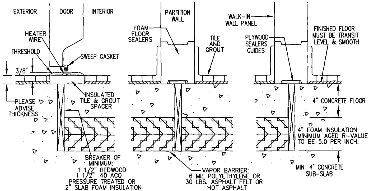
FOAM FLOOR SEALERS ON TOP OF AN INSULATED FLOOR WITH TILE AND GROUT (AFTER WALK-IN INSTALLATION)
