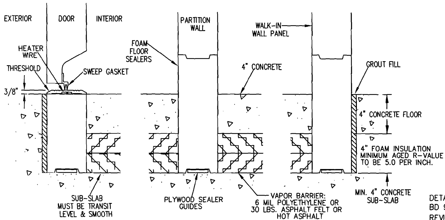
FOAM FLOOR SEALERS USED AS BREAKERS IN AN INSULATED FLOOR (SEALER MUST BE TALLER THAN FINISHED FLOOR)
