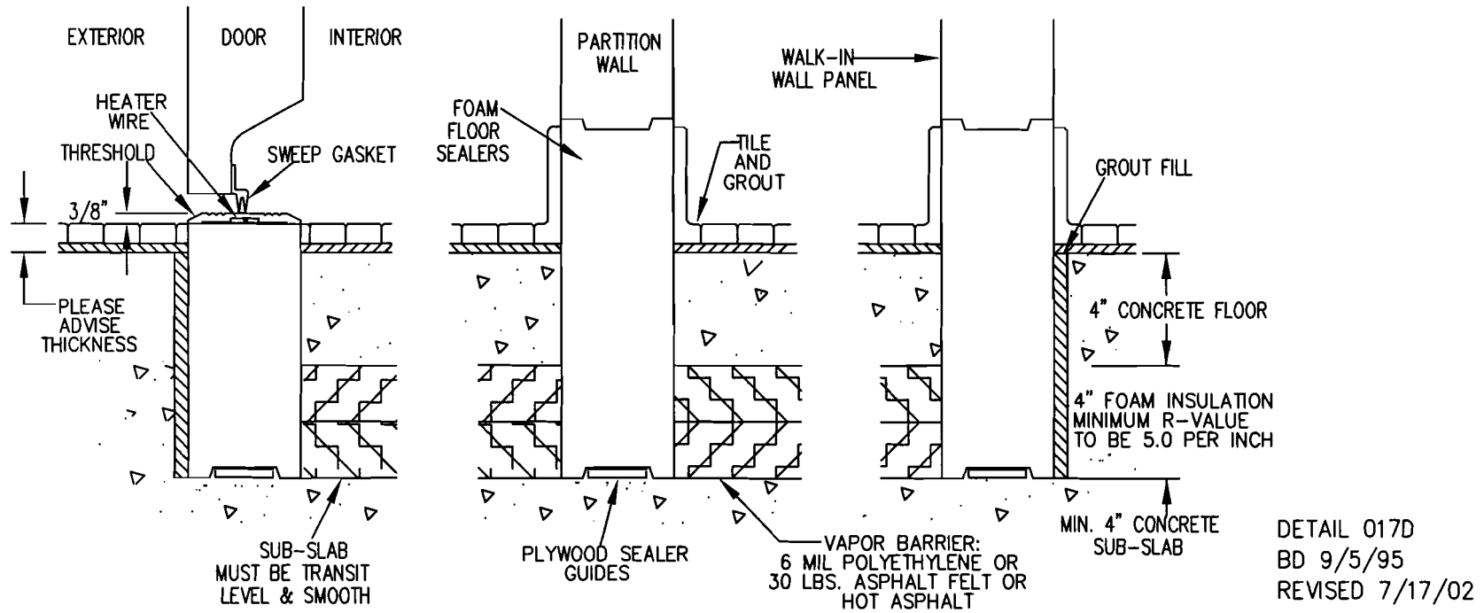
FOAM FLOOR SEALERS USED AS BREAKERS IN AN INSULATED FLOOR WITH A TILE AND GROUT FINISHED FLOOR
