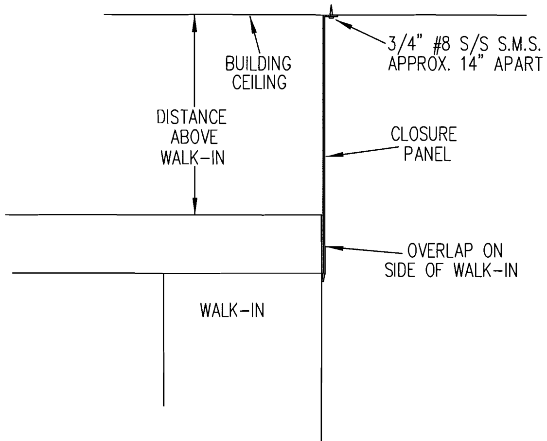
STANDARD CLOSURE PANEL DETAIL
