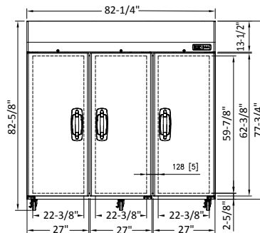
NLTR72-S/NLTF72-S ELEVATION VIEW
