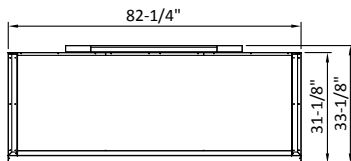
NLTR49-S/NLTF49-S PLAN VIEW
