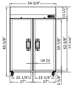
NLTR49-S/NLTF49-S ELEVATION VIEW
