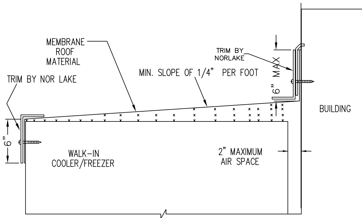
(ELEVATION VIEW) WALK-IN MEMBRANE ROOF TRIM
